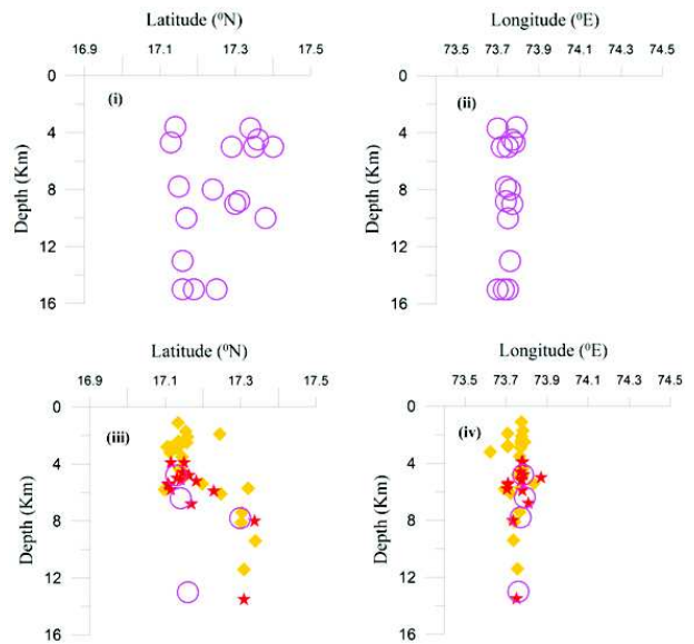
Fig. 1B: Depth section of M ~ 5 earthquakes (epicenters shown in (A) along latitudes (i) and longitudes (ii); and depth sections of M \geq 3.5 earthquakes along latitude (iii) and longitude (iv). Symbols same as in (Fig. 1A). The concentration of hypocenters along 73.75°E is noticeable that corresponds to Donachiwada Fault (Fig. 7)
